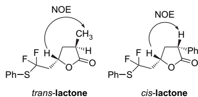
Figure 3. 1 H– 1 H NOESY of trans -lactone and cis -lactone.
