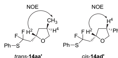
Figure 2. 1 H– 1 H NOESY of trans - 14aa' and cis - 14ad' .
